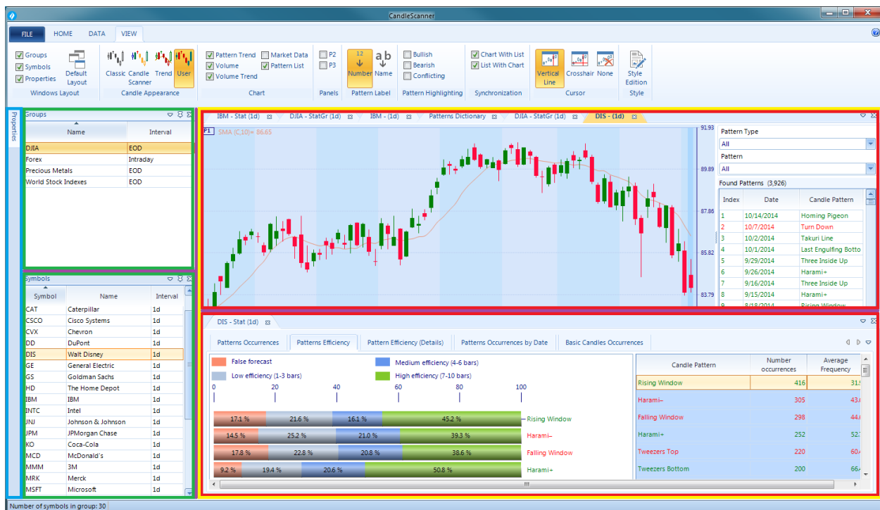
Figure 2.3 Anatomy of CandleScanner windows. Tool windows are in green rectangles (called tool tab strips ). In the yellow rectangle there is a document window container which is divided by a splitter bar (violet line). We can see two document tab strips (red rectangles). Tool windows can be docked on the document window container, but the opposite is not possible. The blue rectangle is used for auto-hiding tool windows.
