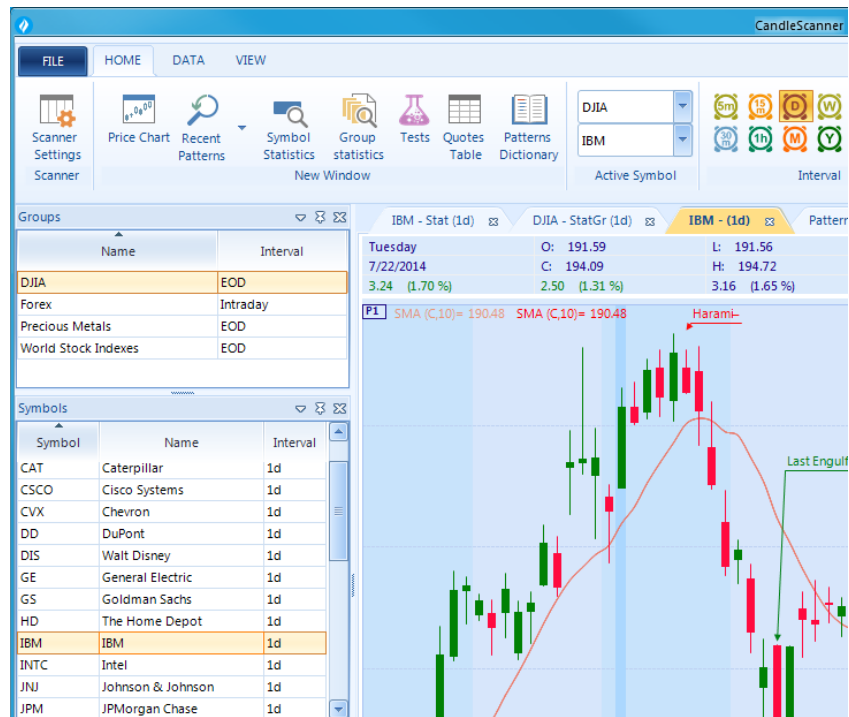
Figure 2.2 Clicking on the DJIA item in the Groups tool window causes the reloading of the DJIA components in the Symbols tool window, which then displays the DJIA components (symbols), as shown. Additionally, the currently active document window, which contains the candlestick chart, is also refreshed and plots the selected symbol, IBM in this case.
